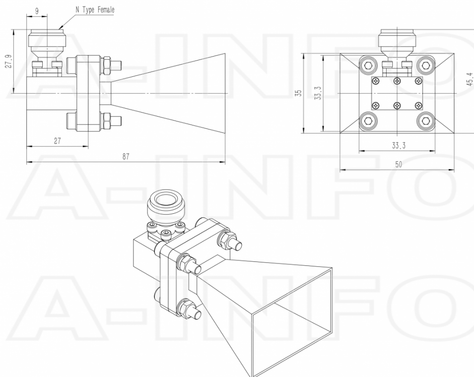
N Type Female Output (P/N: LB-62-15-C-NF)
