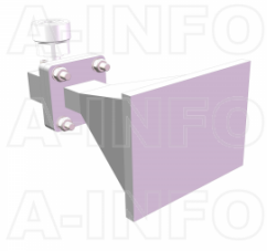
LB-62-15-C-7SPO Standard Gain Horn Antenna 12.4-18GHz 15dB Gain 7mm
