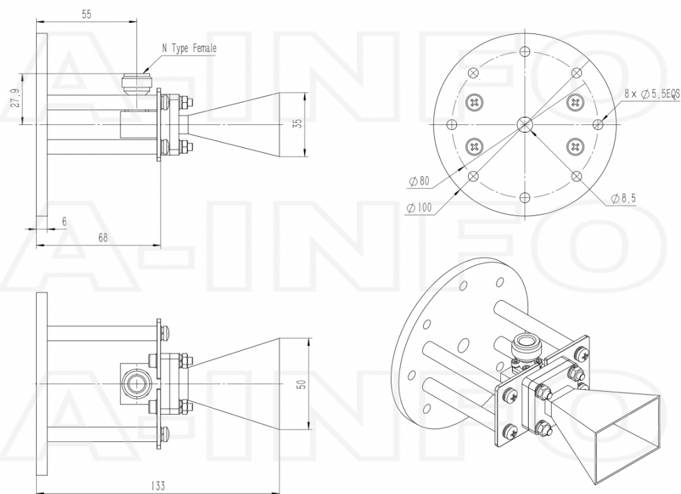
N Type Female Output with Round Mounting Bracket (Option, P/N: LB-62-10-C-MB)
